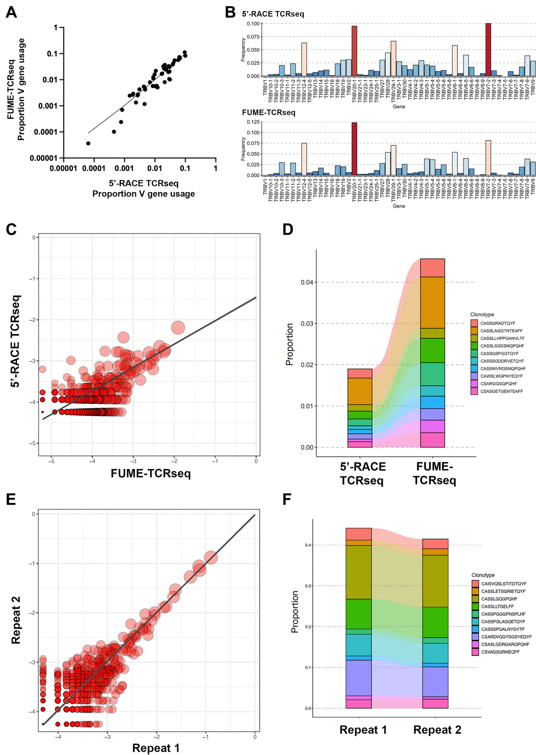
Figure 2. A , Scatter plot showing V gene usage data from FUME-TCRseq and 5'-RACE ligation ("5'-RACE TCRseq") methodologies, performed on RNA extracted from a representative whole blood sample. B , Bar plot showing the proportion of each V gene detected by FUME-TCRseq and 5'-RACE ligation. Red bars, highly frequent V genes; blue, less frequent V genes. C , Scatterplot showing overlapping clonotype abundances for the FUME-TCRseq and 5'-RACE TCRseq data. Point size is scaled to the geometric mean of clonotype frequency in both samples and axes represent \log_{10} clonotype frequencies in each sample. D , Plot showing the 10 most common clonotypes identified by FUME-TCRseq and the frequencies at which they were detected using 5'-RACE ligation methodology. E , Scatterplot showing overlapping clonotype abundances for technical repeats. Point size is scaled to the geometric mean of clonotype frequency in both samples and axes represent \log_{10} clonotype frequencies in each sample. F , Plot showing the 10 most common clonotypes detected in technical repeats of FUME-TCRseq performed on RNA extracted from an inflammatory polyp.
